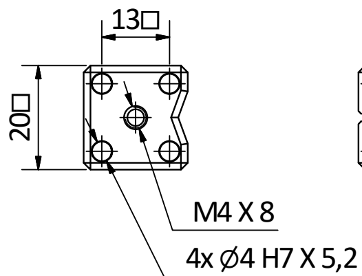
FT 20-UNI
